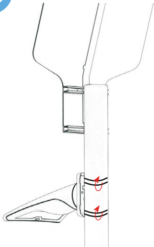
Secure mounting post using Jubilee Clips (not supplied) and tighten
